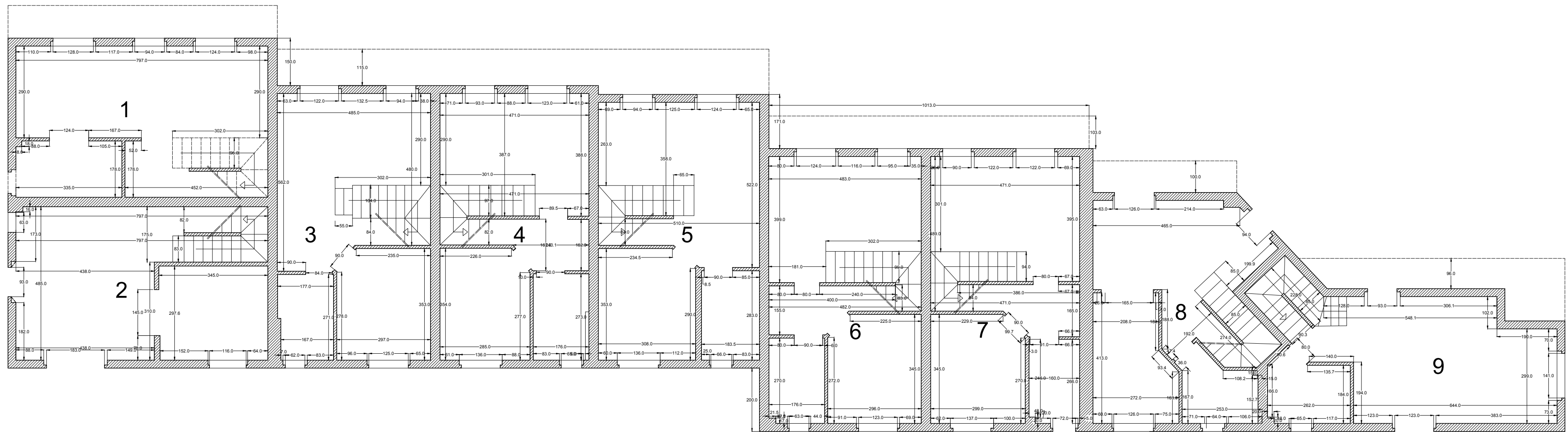
PIANO TERRA
