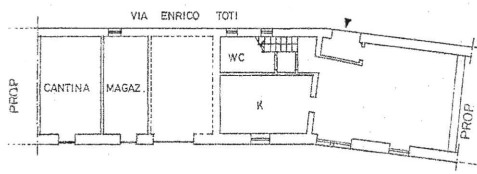
PIANO TERRENO H = 2.95
