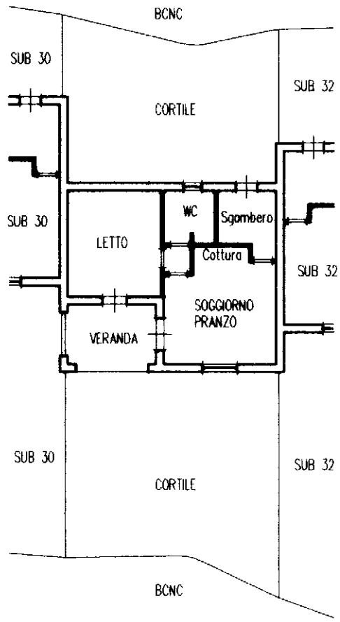
PIANO TERRA H=2.70
