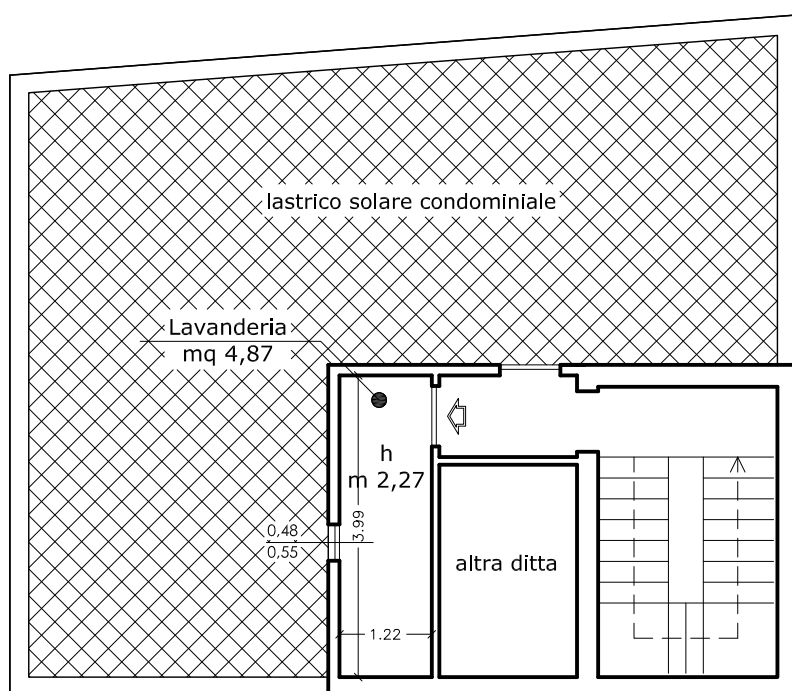
Piano quarto
