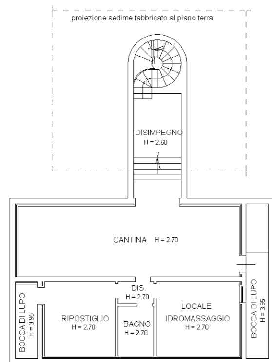
PIANO INTERRATO
