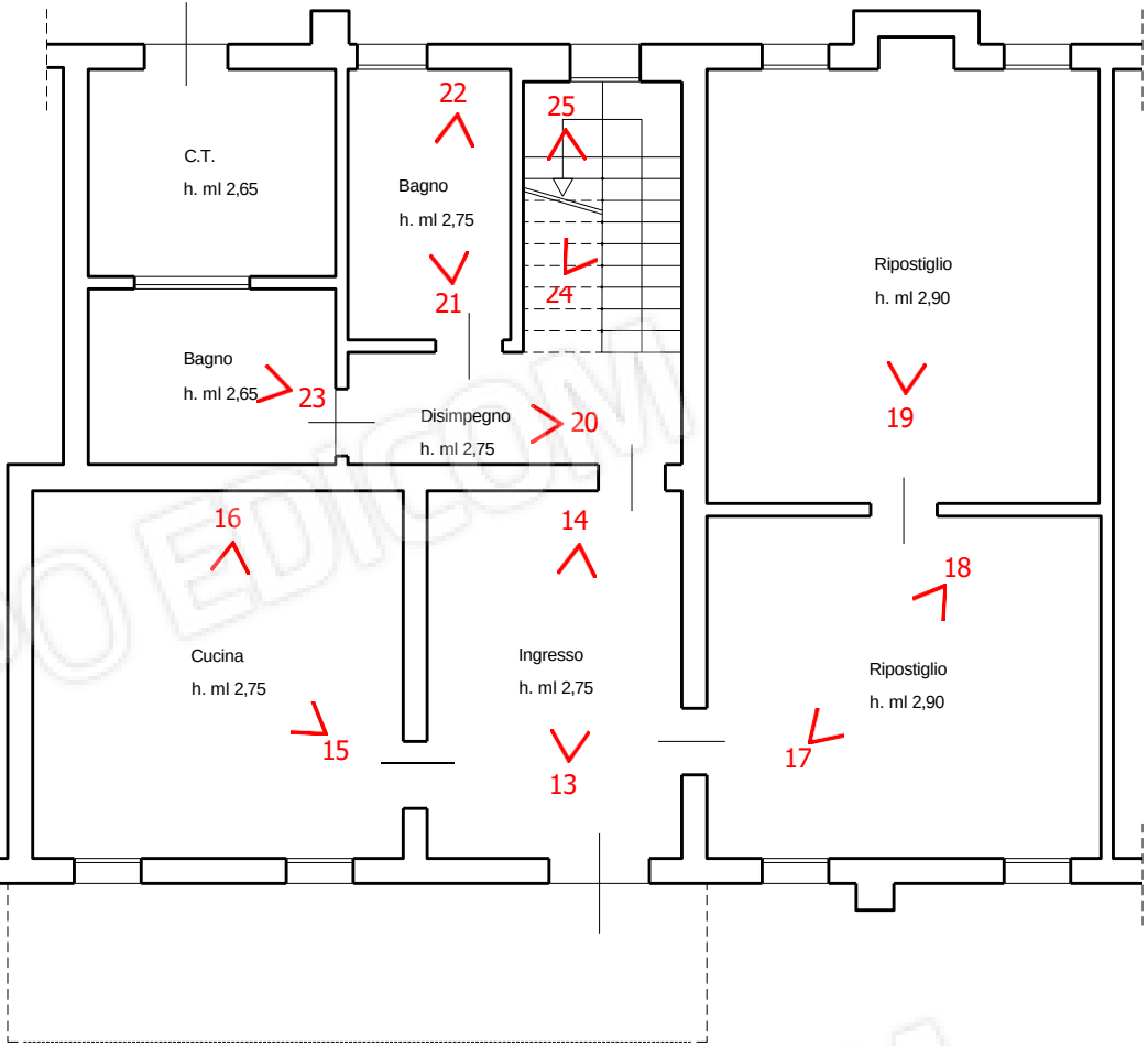
Piano Terra
