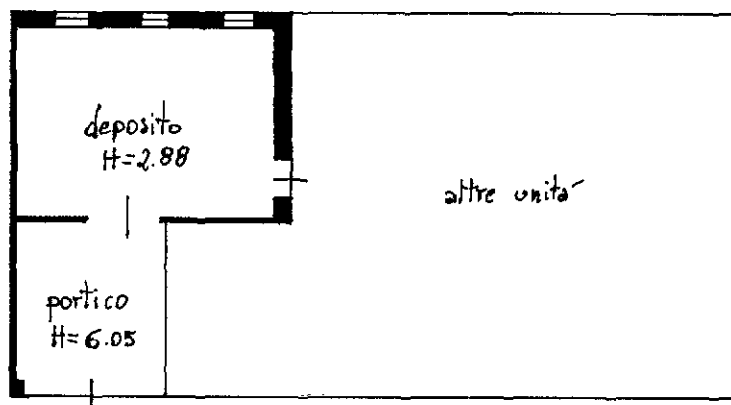
PIANO TERRA
