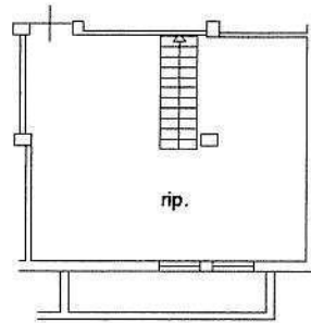
Pianta piano interrato H 2.50m
