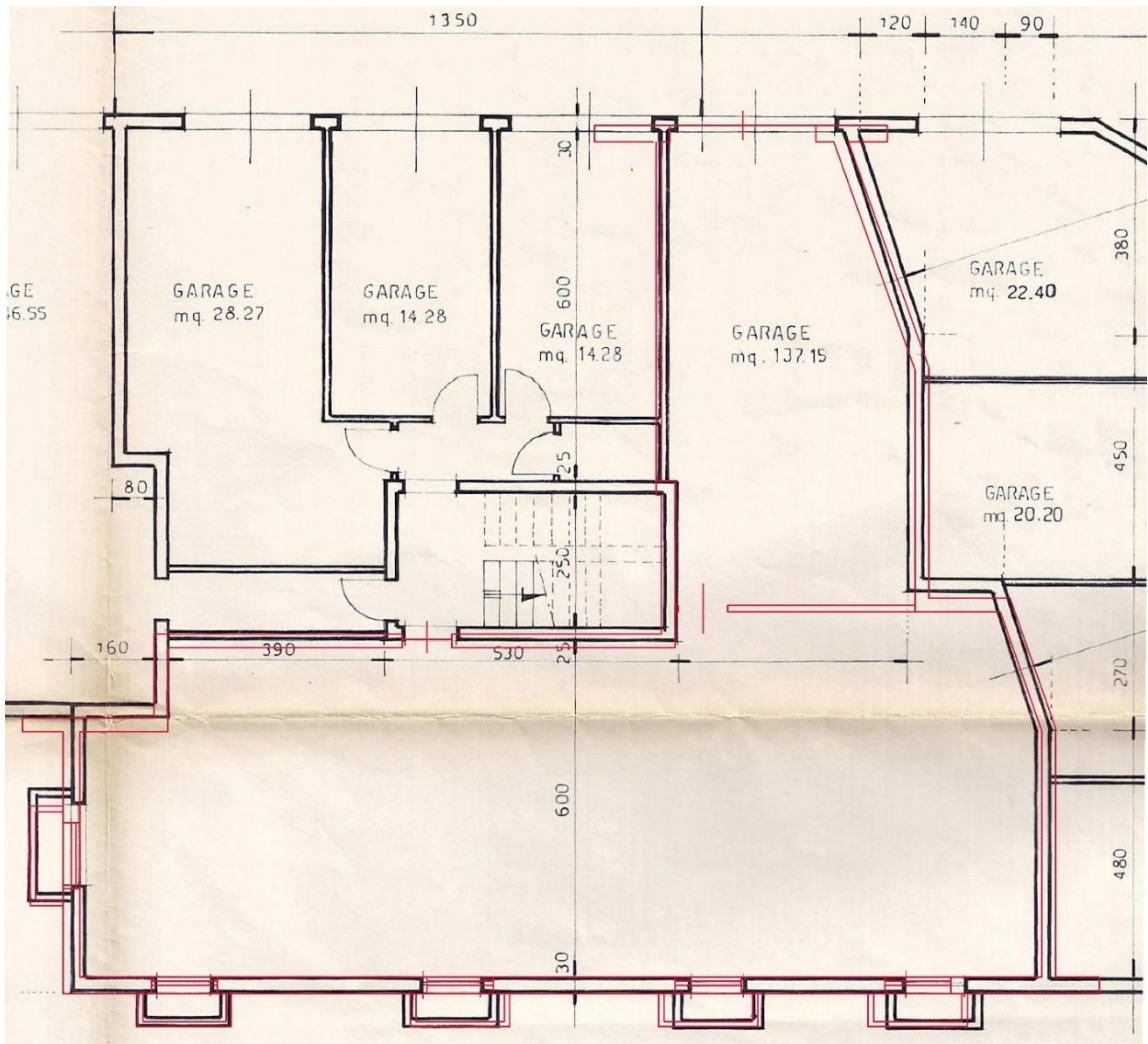
PIANO INTERRATO
