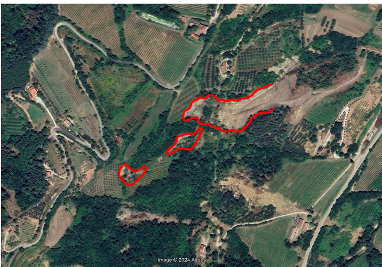
In evidenza le aree alluvionate e franate post 2023
