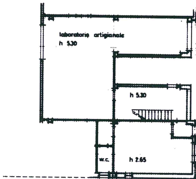
PIANO TERRA
