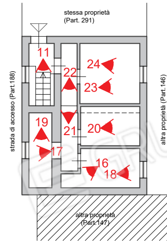
PIANO TERRA (Part.148 sub 3)
