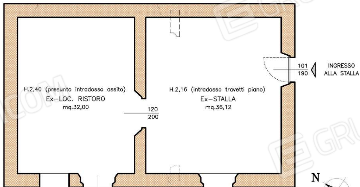
PIANO TERRA
