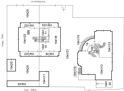
PIANO TERRA
