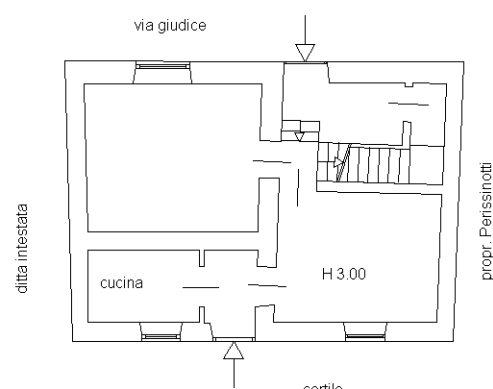
Piano Terra
