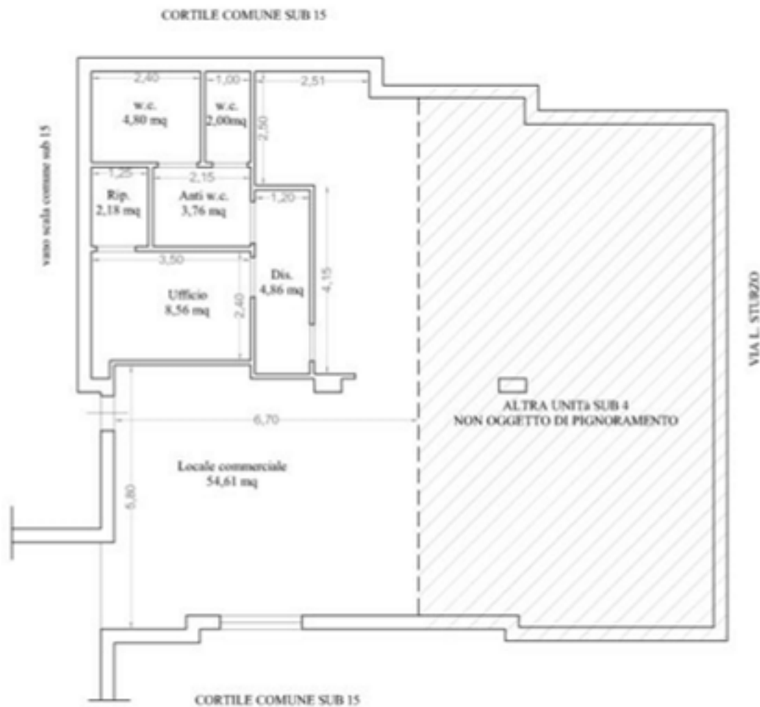
PIANTA PIANO TERRA H=3,55m
